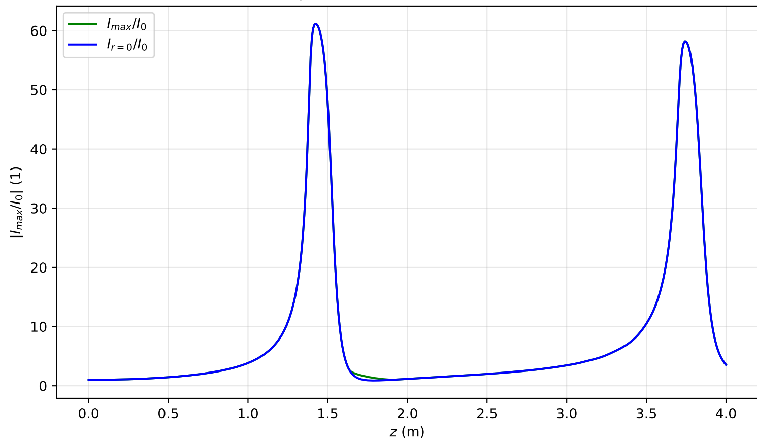
I_{max}(x = 0, y = 0, z)/I_0 , P_{in}=1.7P_{cr} , artificial time
